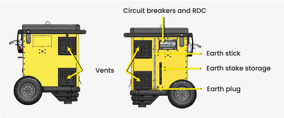
Figure 3 : Lateral surfaces of the device
