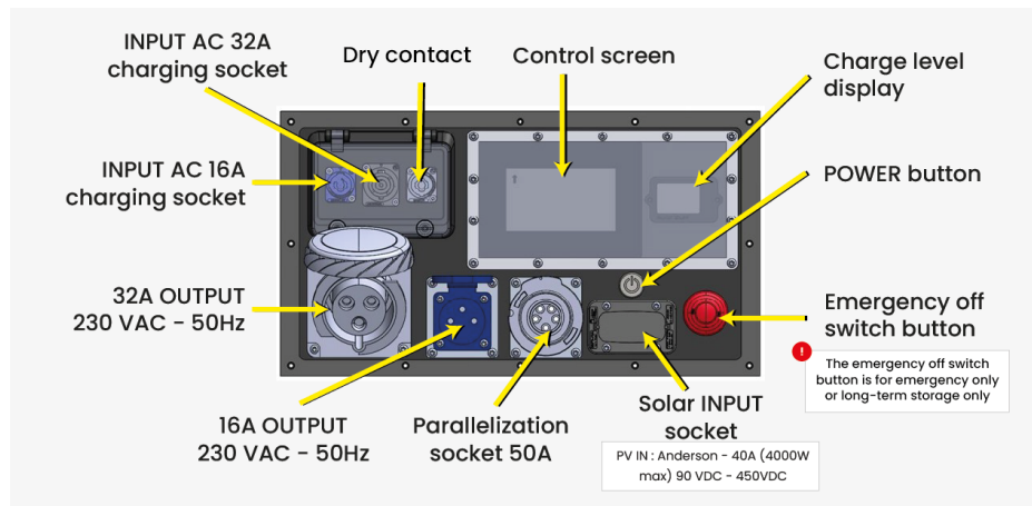
Figure 1 : Sockets layout
