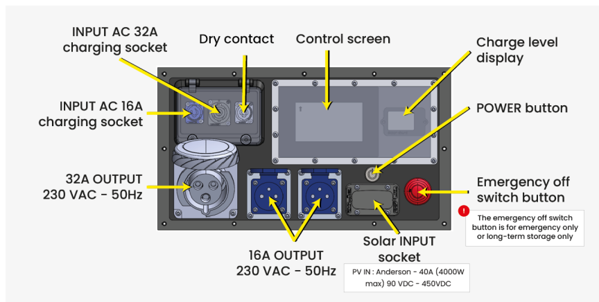
Figure 1: Sockets layout
