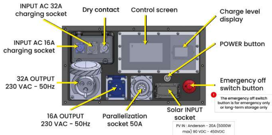
Figure 1: Sockets layout
